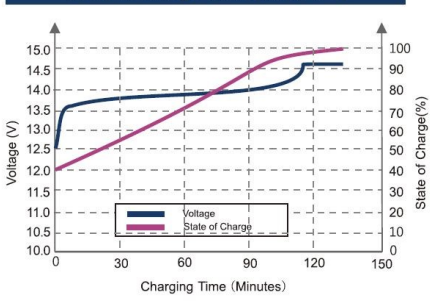
State of Charge Curve(0.5C, 25°C)
